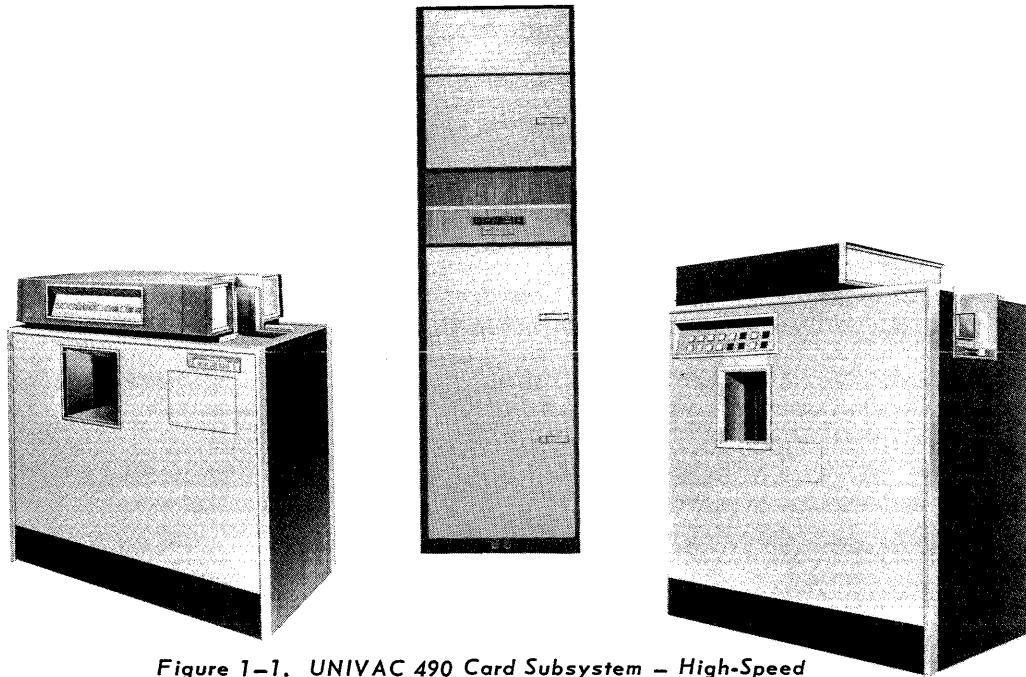
Figure 1-1. UNIVAC 490 Card Subsystem – High-Speed Reader, Channel Synchronizer-Control Unit and Punch Verifier
