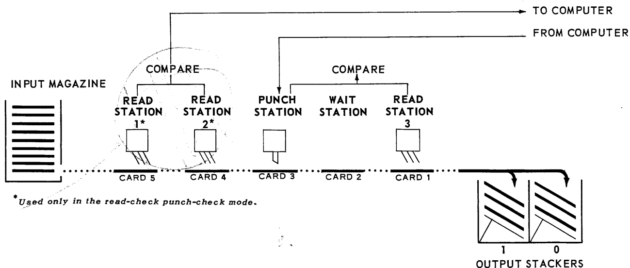
Figure 2-1. Punch-Verifier Transport System
