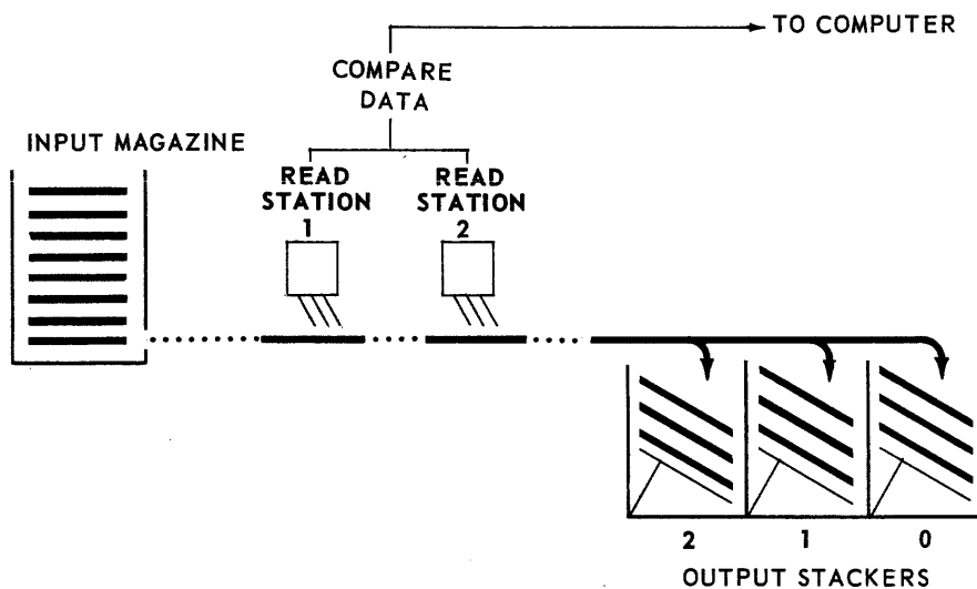
Figure 2-2. High-Speed Reader Transport System
