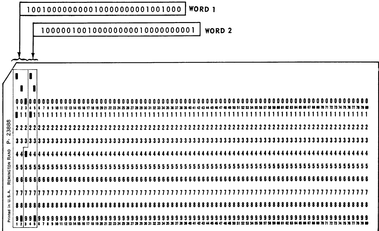
Figure 3-2. Relationship of Computer Words to Card Punches (by Column)
