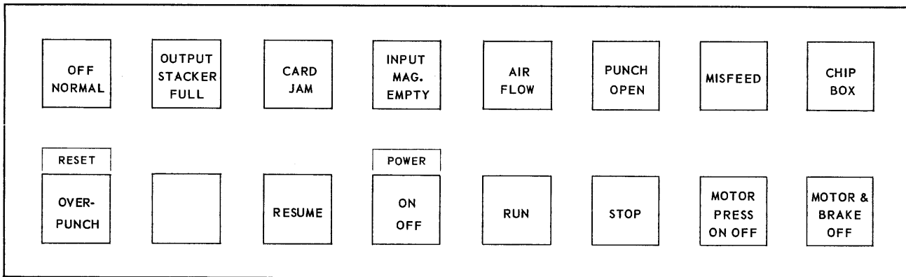
Figure 4-2. Punch Verifier Control Panel
